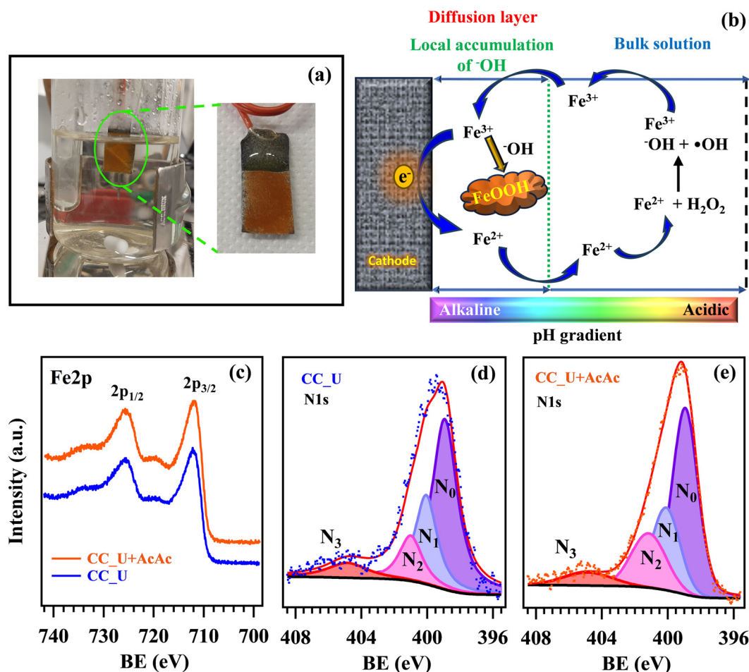
Fig. 8 (a) Image of the CC_U + AcAc sample after the test for 24 h as a working electrode in EF processes for FNT degradation. (b) Sketch of the route yielding insoluble \text{Fe}(\text{III}) deposits onto the electrode's surface. XPS signals after EF tests for Fe2p (c) and N1s (d and e).
