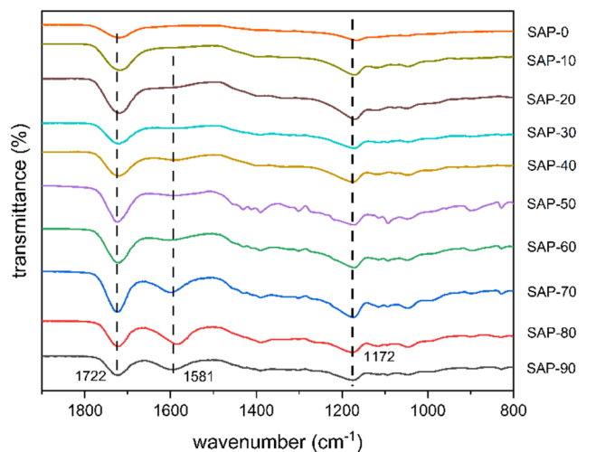
Fig. 4 FTIR spectra of extracted SAPs synthesized from CA, MSC, and GLY and after thermal cross-linking. Molar feed ratio of (CA + MSC)/GLY is always 1/1, weighed in molar monomer ratios CA/MS ( %ND) indicated in the figure.
