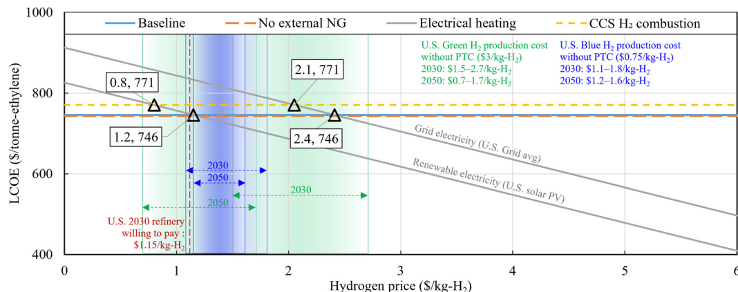
Fig. 14 Impact of hydrogen price on LCOE of ethylene production.
