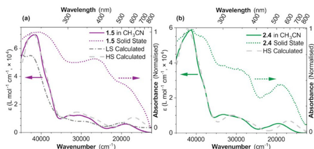
Fig. 7 (a) UV-visible spectra of 1.5 in solution and the solid state along with the calculated spectra for the optimised LS and HS [\text{Fe}^{\text{III}}(5\text{-I-sal}_2232)]^+ cation (B3LYP/def2-TZVP/D3BJ). (b) UV-visible spectra of 2.4 in solution and the solid state along with the calculated spectra for the optimised HS [\text{Fe}^{\text{III}}(5\text{-I-sal}_2232)]^+ cation (B3LYP/def2-TZVP/D3BJ). All spectra were recorded at room temperature.
