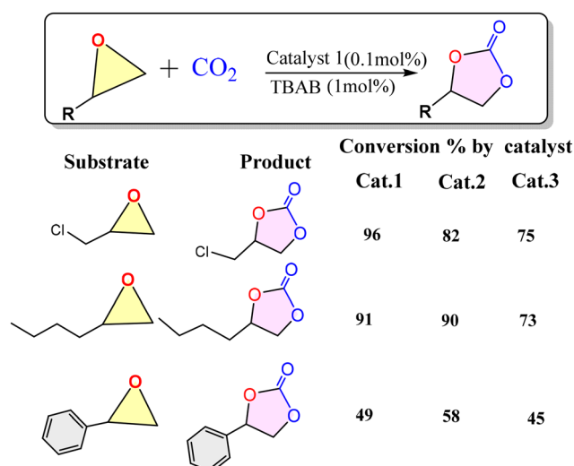
Scheme 5 Cycloaddition reaction of \text{CO}_2 with different epoxides to form cyclic carbonates by using catalysts 1-3.
