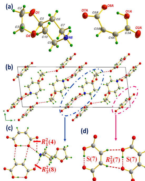
Fig. 6 Asymmetric unit of compound III (a), projection of the structure along the ( \vec{a} , \vec{c} ) plane (b) marking the formation of R_3^2(8) and R_1^2(4) supramolecular synthons between anions and cations (c), intra- and intermolecular S(7) and R_3^2(7) interaction motifs formed between MAs (d).
