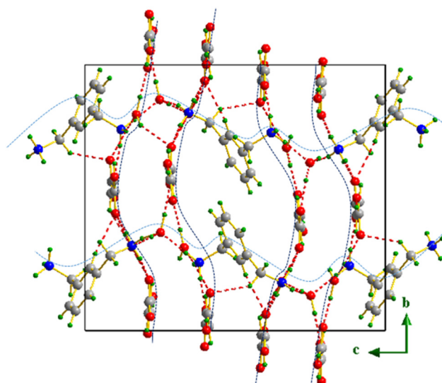
Fig. 17 Molecular packing of m -xylylenediamine/fumaric acid-trihydrate salt (VI) along the ( b , c ) plane.
