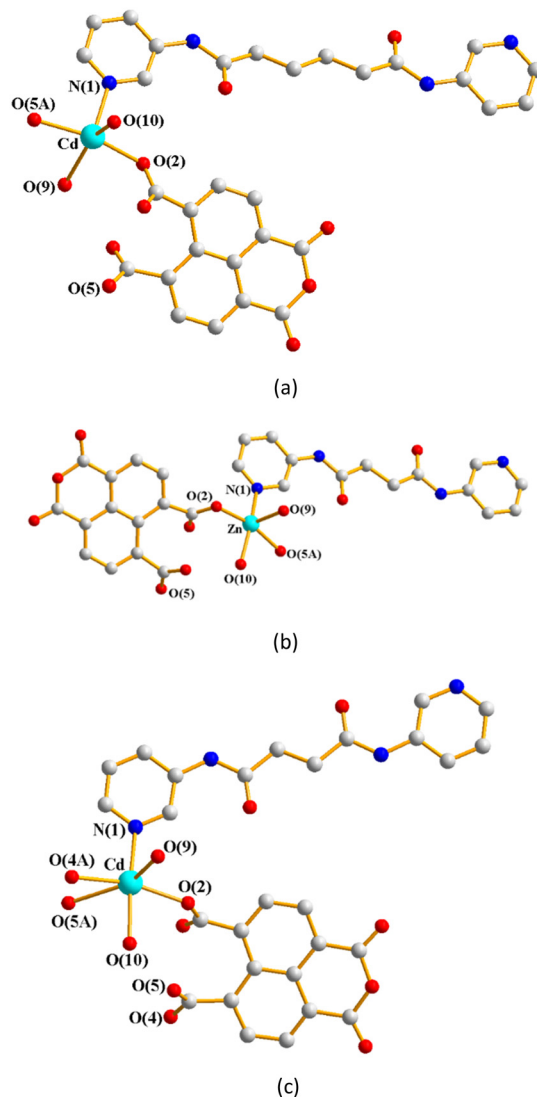
Fig. 4 (a) Coordination environment about the \text{Cd}(\text{II}) ion of 1. Symmetry transformations used to generate equivalent atoms: (A) -x, -y + 2, -z + 2 . (b) Coordination environment about the \text{Zn}(\text{II}) ion of 2. Symmetry transformations used to generate equivalent atoms: (A) -x - 1, -y + 2, -z + 1 . (c) Coordination environment about the \text{Cd}(\text{II}) ion of 3. Symmetry transformations used to generate equivalent atoms: (A) -x + 1, -y + 1, -z .
