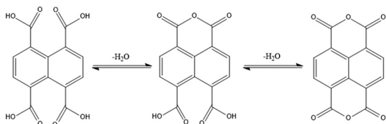
Fig. 2 Condensation pathways from 1,4,5,8- \text{H}_4\text{NTC} to 1,4,5,8- \text{H}_2\text{NTC}' and \text{NTC} .
