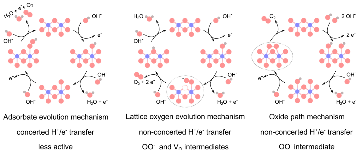
Scheme 1 Proposed mechanisms for the alkaline OER. Co atoms are shown in blue, O in red, H in grey, and oxygen vacancies ( V_{\text{O}} ) in dashed red circles. The characteristic steps with superoxide \text{OO}^- intermediates are indicated with grey dashed ellipses. Scheme inspired by Rong et al. 14
