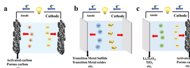
Fig. 2 Schematic diagram of the energy storage mechanisms of (a) EDLCs, (b) PCs, and (c) HSCs.
