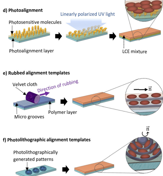
Fig. 7 LCE alignment methods: (1) bulk alignment: (a) electric field: the director aligns with the electric field direction. (b) Magnetic field: mesogens align with the magnetic induction intensity direction. (c) Mechanical stresses: alignment direction follows the stretching direction. (2) Photoalignment: the director can be perpendicular or parallel to the light vector's direction. (2) Interfacial alignment: (e) rubbed alignment templates: the direction of mechanical friction during rubbing defines the alignment direction of the mesogens. (f) Photolithographic alignment templates: microchannel direction dictates the alignment of mesogens within the LCE.
