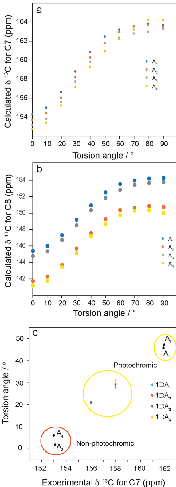
Fig. 5 DFT-calculated 13 C chemical shifts of (a) C7 and (b) C8 in single molecules of A 1 –A 4 compounds at fixed torsion angles. (c) Correlation of torsion angles in crystal structures of A 1 –A 4 against experimental 13 C chemical shift of C7 (black dots). Also shown are points representing predicted torsion angles for A 1 –A 4 within 1 ⊃A n host–guest complexes based on the calculated torsion angle dependence of the C7 chemical shift derived from the plot in (a) (coloured dots).
