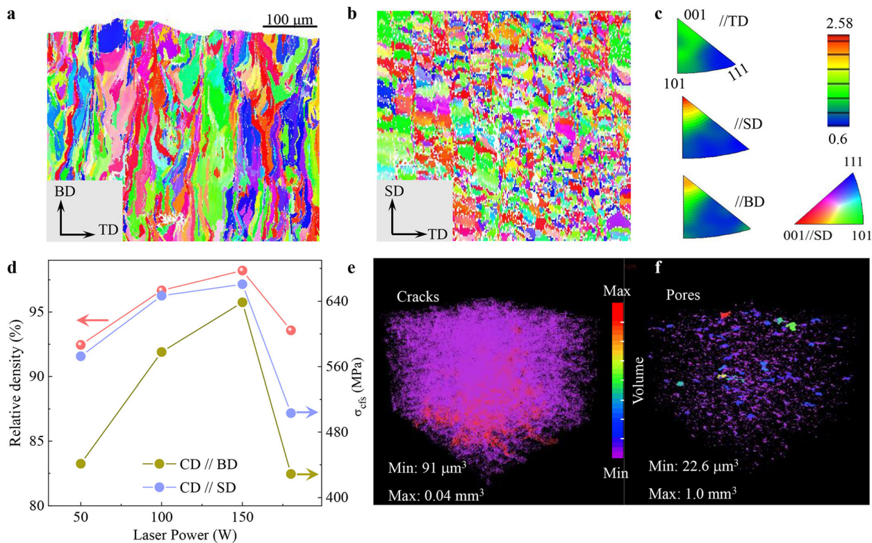
Fig. 3 EBSD mapping of sample P 180 in the (a) building-transverse direction (BD-TD) and (b) transverse-scanning direction (TD-SD) planes. (c) The inverse pole figures show (001) texture along the SD and BD. All the inverse pole figures are plotted with the (001) directions parallel to the SD. (d) Relative density and fracture stress after cycling loading ( \sigma_{cfs} ) in L-PBF Ni–Mn–Sn alloys prepared with different laser powers. 3D reconstructed morphology of cracks (e) and pores (f) via Mico-CT in P 150 samples. The different colors represent the difference in the volume of cracks and pores.
