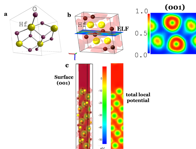
Fig. 2 Structure of hafnium oxide (monoclinic phase P 2 1 / c ); (a) crystalline structure; (b) electron localization function (ELF) of a (001) slice; ELF = 1 and ELF = ½ corresponding to the localized and electron gas; (c) total local potential of a surface (001) of HfO 2 .
