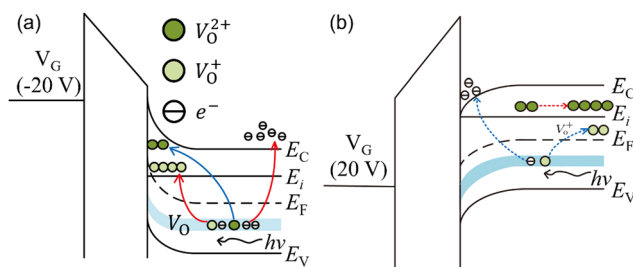
Fig. 14 Schematic energy-level diagrams of AOS TFTs under stresses of (a) NBIS and (b) PBIS, and the generation of V O + and V O 2+ . Reproduced with permission. 126 Copyright 2024, Chinese Physics B.
