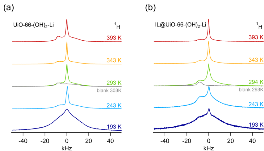
Fig. 7 Variable-temperature ^1\text{H} NMR lines (300 MHz) of UiO-66-(OH) _2 -Li and IL@UiO-66-(OH) _2 -Li. As ^1\text{H} possesses the highest relative sensitivity of all NMR nuclei and because protons are ubiquitous in the surrounding atmosphere and the probe head, two blank ^1\text{H} NMR lines (without a sample in the NMR coil) were acquired. (a) Grafted UiO-66-(OH) _2 -Li in pure form showing little motional narrowing of the NMR line above 243 K. (b) IL@UiO-66-(OH) _2 -Li ionogel consisting of grafted UiO-66-(OH) _2 -Li MOF with added EMIM-FSI ionic liquid. While there are mobile protons at all temperatures, the relative ratio between fast and slow protons increases significantly with temperature.
