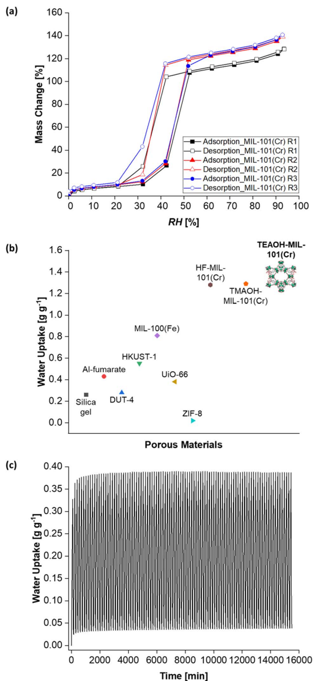
Fig. 7 (a) Water adsorption–desorption isotherms ( T = 25\text{ °C} ) of TEAOH-MIL-101(Cr) where the water uptake capacity increases with additional rounds of washing in warm ethanol. (b) Water uptake of various MOFs at T = 25\text{ °C} and RH = 90%. The water uptake of silica gel under the same conditions is included for comparison. (c) Cyclic performance of TEAOH-MIL-101(Cr) R3 over 100 adsorption–desorption cycles with 90 min of adsorption at T = 25\text{ °C} and RH = 50% followed by 65 min of desorption at T = 50\text{ °C} and RH = 0%.
