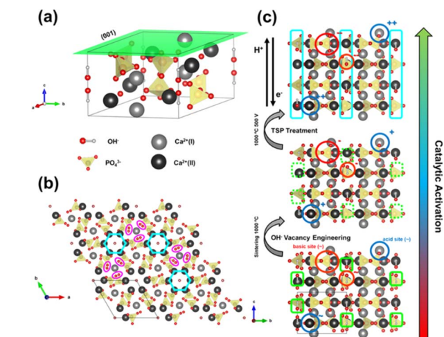
Scheme 1 Structure of HAP as a catalyst. (a) HAP unit cell P6_3/m . (b) (001) crystallographic plane observed from the c -axis direction. The OH - channels and the Ca(i) 6-fold coordination are highlighted. (c) Structural changes and lattice refinement strategies adopted to achieve the catalytic activation of HAP.
