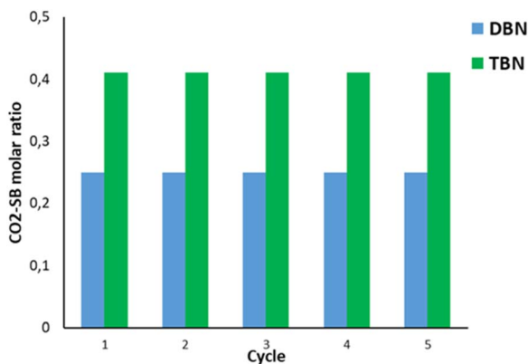
Fig. 5 Five consecutive recycling experiments with (a) TBN in butyl acetate (green) and (b) DBN in acetonitrile (blue).
