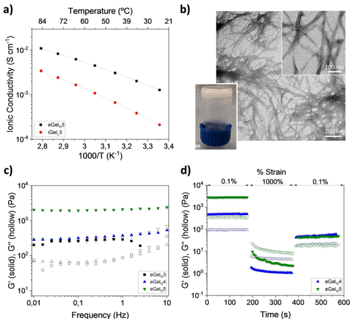
Fig. 8 (a) Ionic conductivity of the eutectogel eGel G 3 and the iongel iGel 3 at different temperatures. (b) TEM image of the eutectogel eGel G 3. (c) Storage modulus ( G' ) and loss modulus ( G'' ) as a function of the frequency of the eutectogels eGel G 3, eGel G 4 and eGel G 5. (d) Dynamic step-strain amplitude tests of eGel G 4 and eGel G 5 eutectogels. Reprinted from M. Criado-Gonzalez, N. Alegret, A. M. Fracaroli, D. Mantione, G. Guzmán-gonzález, R. Del Olmo, K. Tashiro, L. C. Tomé, M. L. Picchio and D. Mecerreyes, Mixed Conductive, Injectable, and Fluorescent Supramolecular Eutectogel Composites, Angew. Chem., Int. Ed. , 2023, 62, e202301489 (Creative Commons Attribution 4.0 International License CC BY-NC-ND 4.0 http://creativecommons.org/licenses/by/4.0/ ).
