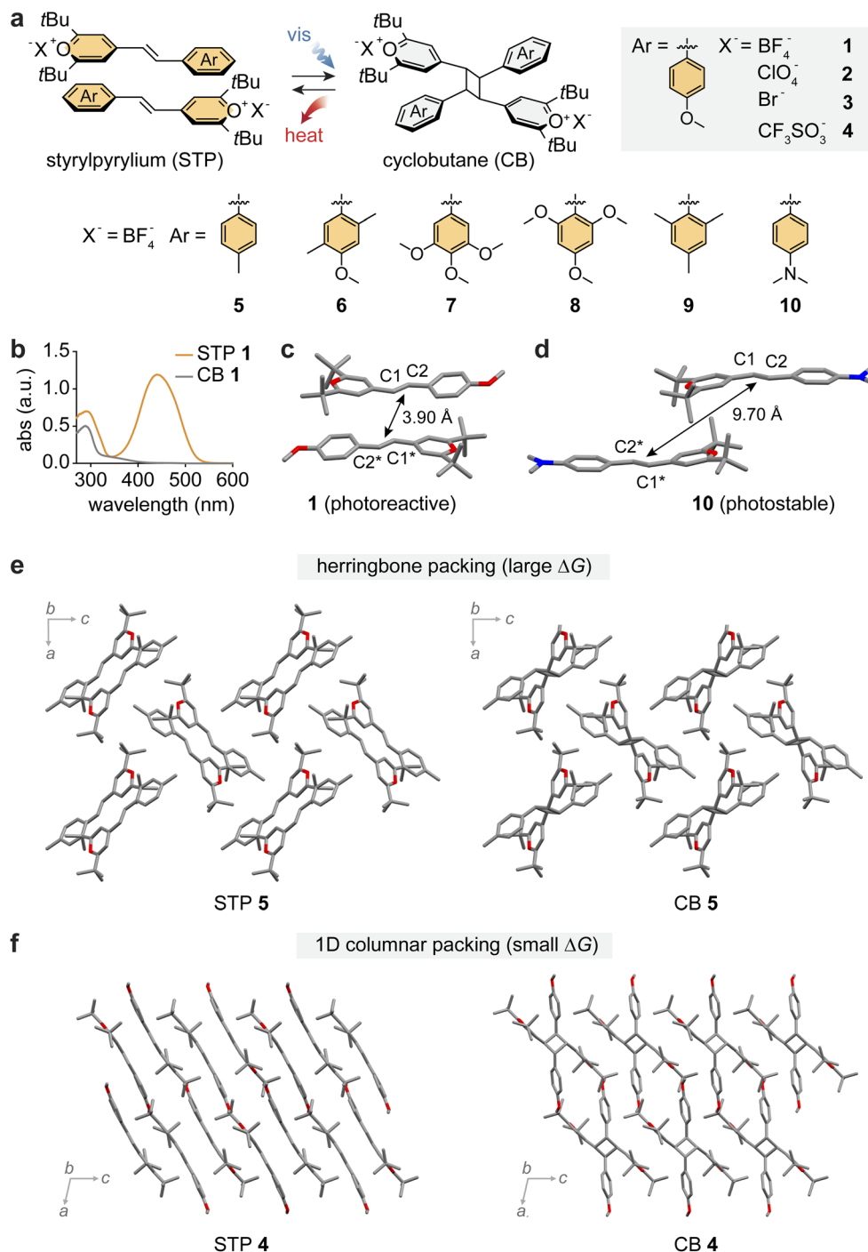
Fig. 3 (a) Reversible photoinduced [2 + 2] cycloaddition and reversion between styrylpyrylium (STP) and cyclobutane (CB) with varied functional groups on the phenyl ring and varied counter-anions ( \text{X}^- ). (b) UV-vis absorption spectra of STP 1 (orange) and CB 1 (gray). Crystal structures of (c) STP 1 showing proximal head-to-tail packing for [2 + 2] cycloaddition and (d) STP 10 showing offset packing unsuitable for cycloaddition. Crystal packing structures of (e) STP 5 and CB 5 and (f) STP 4 and CB 4 representing herringbone and 1D columnar packing, respectively. In panels (c)–(f), the hydrogen atoms are omitted in the crystal packing for clarity. This figure has been reproduced from ref. 44 with permission from Elsevier, copyright 2023.
