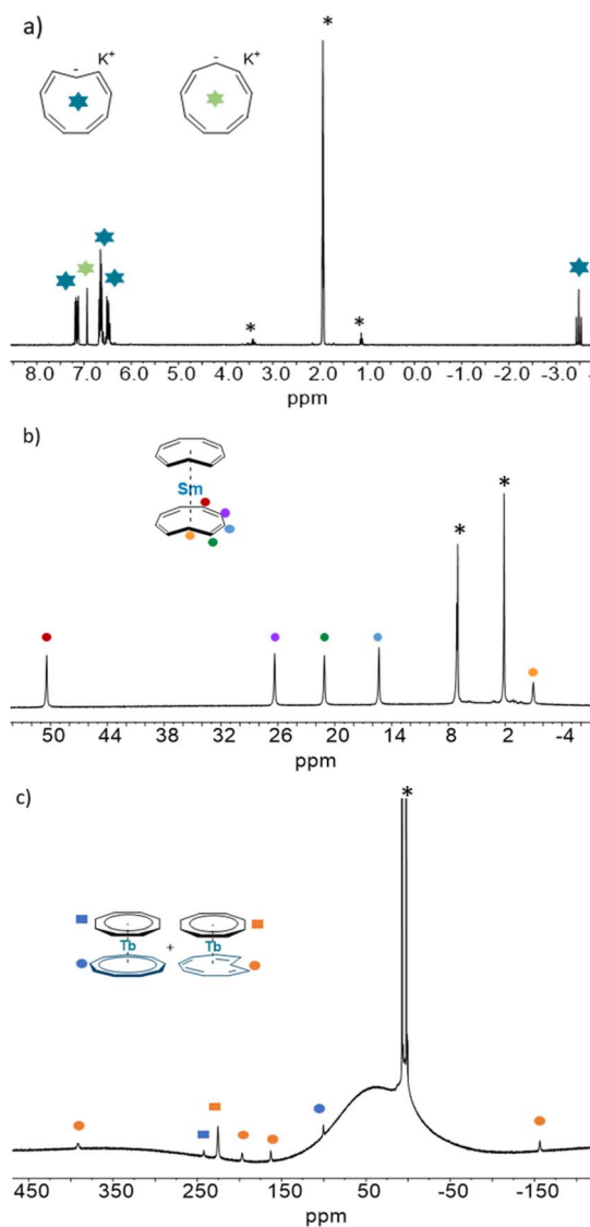
Fig. 4 ^1\text{H} NMR of the (a) cis/trans \text{KC}_9\text{H}_9 , of (b) 1\text{-trans} and of (c) 2\text{-Tb-trans} .
