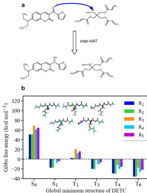
Fig. 6 Radical reaction mechanisms between DETC and PETA. (a) HAT reaction between DETC in a high triplet state and PETA in the ground state that leads to the formation of a ketyl radical on DETC and an alkyl radical on PETA (R 1 or R 2 ) that consequently initiates the polymerization (R 1 is reported in the figure). It is important to note that all carbon atoms in the alpha position with respect to the central carbon atom in the pentaerythritol fragment of PETA are equally susceptible to form radicals. (b) Gibbs free energy of the reaction involving different PETA radicals (R 1 –R 5 , see Fig. S18†) as a function of the electronic state of DETC (see Table S24†). Energies were computed employing (U)CAM-B3LYP-D3(BJ)/def2-TZVP approach in implicit ACN.
