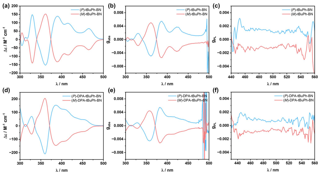
Fig. 6 (a) CD spectra and (b) g_{\text{abs}} values of tBuPh-BN recorded in 5 \times 10^{-6} mol L ^{-1} toluene solution. (c) g_{\text{PL}} values of tBuPh-BN recorded in 10^{-5} mol L ^{-1} THF solution. (d) CD spectra and (e) g_{\text{abs}} values of DPA-tBuPh-BN recorded in 5 \times 10^{-6} mol L ^{-1} toluene solution. (f) g_{\text{PL}} values of DPA-tBuPh-BN recorded in 10^{-5} mol L ^{-1} THF solution.
