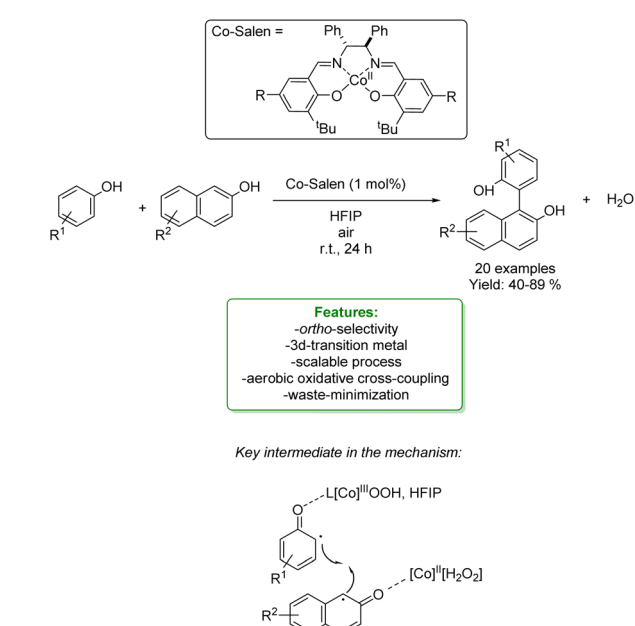
Scheme 74 Co-catalysed phenol–phenol cross-coupling. 212
