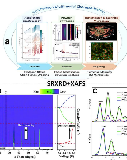
Fig. 14 Synchrotron multimodal characterization for the study of cathode materials in AZIBs. (a) Multi-modal X-ray synchrotron characterization of the energy storage mechanism of the MnO 2 cathode. Adapted from ref. 160, copyright 2023, The Royal Society of Chemistry. (b) Operando SXR D spectra of the MnV 2 O 4 @C cathode during cycling; (c) Mn and Zn EXAFS spectra of the MnV 2 O 4 @C cathode in different states. Adapted from ref. 155, copyright 2021, The Royal Society of Chemistry.
