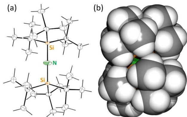
Fig. 1 (a) ORTEP representation for the crystal structure of (t\text{Bu}_3\text{Si})_2\text{NH} ( t^{\text{Bu}}\text{NH} ). The H atom at N is disordered and was not located. (b) Space-filling model for the crystal structure of (t\text{Bu}_3\text{Si})_2\text{NH} ( t^{\text{Bu}}\text{NH} ).
