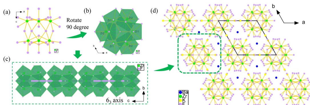
Fig. 1 (a and b) \text{cis-}[\text{Zr}_6\text{F}_{34}]^{10-} cluster at the ac and ab plane; (c) the \{\{\text{Zr}_6\text{F}_{34}\}^{10-}\}_\infty chain along the c -axis; (d) the aligned arrangement of the \{\{\text{Zr}_6\text{F}_{34}\}^{10-}\}_\infty anionic chains and whole structure of \text{K}_3\text{Ba}_2\text{Zr}_6\text{F}_{31} viewed along the c -axis.
