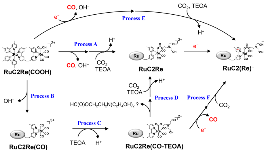
Scheme 3 Subsequent processes of \text{RuC2Re(COOH)} .
