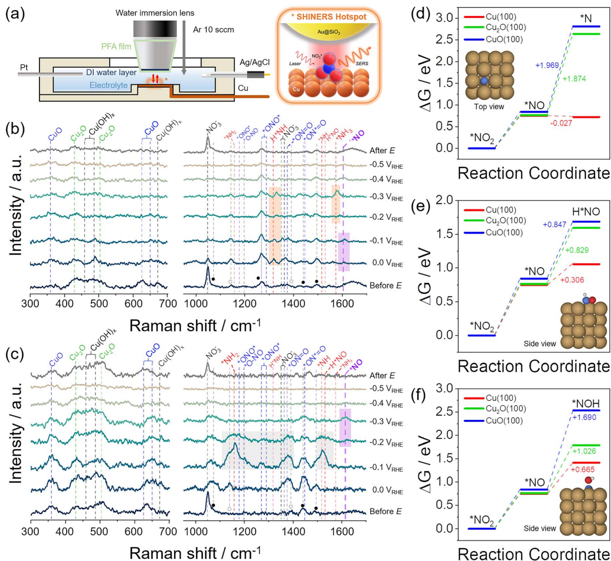
Fig. 4 Operando SHINERS analysis for NO 3 - reduction process on e-Cu and w-Cu electrodes. (a) Schematic illustration of an electrochemical cell. The right scheme illustrates the SERS hotspot by the SHIN (Au@SiO 2 ) particle placed on top of the Cu surface undergoing a chemical reaction. (b and c) SERS spectra for (b) e-Cu and (c) w-Cu, before the test, 0.0 V—0.5 V vs. RHE, and after the test (from bottom to top). The potential was negatively scanned with -100 mV step. Vertical dashed lines indicate vibrational frequencies of CuO, Cu 2 O, Cu(OH) x , NO 3 - (black), NO 2 - (blue), NO (violet), HNO/NH/NH 2 /NH 3 (red). For the details of peak assignment, see Tables S4 and S5.† The orange, violet, and gray box indicate *NH 2 /*NH 3 , *NO, and byproduct intermediates, respectively. (d–f) Reaction free energy diagrams of (d) *NO 2 → *N, (e) *NO 2 → H*NO, and (f) *NO 2 → *NOH on Cu(100), Cu 2 O(100), and CuO(100) at pH = 14, calculated by DFT. The insets showed the optimized structures of three final intermediates adsorbed on Cu(100) (brown, blue, red, and white represent Cu, N, O, and H, respectively).
