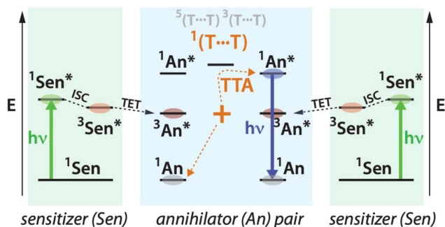
Scheme 1 Representation of TTA-UC with relevant states and processes central to determination of upconversion yield \phi_{\text{UC}} . The intermolecular multiexciton singlet is shown as mediating the TTA event but other excited states can also be involved.
