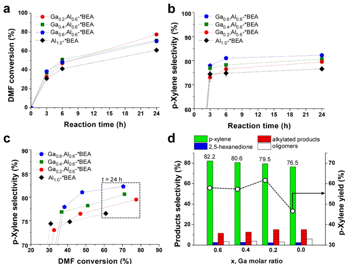
Fig. 3 Tandem Diels-Alder/dehydration reaction performance of *BEA catalysts at 250 °C and 60 bar: (a) DMF conversion (starting from 0.23 M DMF in heptane) and (b) p-xylene selectivity vs. reaction time; (c) p-xylene selectivity vs. DMF conversion; and (d) products selectivities (histograms, left y-axis) and p-xylene yield (open circles, right y-axis) after 24 h of reaction. The x-axis lists the Ga molar ratio for each \text{Ga}_x\text{Al}_{0.6}\text{-*BEA} catalyst. Dashed lines are interpolated to guide the eye. Symbols are the average of three measurements for a single experiment. Error bars span two standard deviations (those not visible are less than the size of the symbol). This error is in good agreement with reproducibility tests that compared separate reactions in triplicate for the \text{Al}_{1.0}\text{-*BEA} catalyst (see Fig. S10 of the ESI†).
