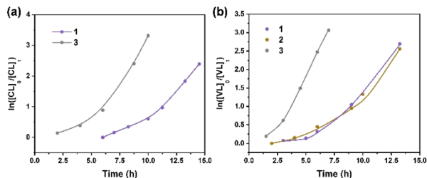
Fig. 7 (a) Plot of \ln([CL]_0/[CL]_t) vs. time for the polymerization of \epsilon -CL initiated by 1 and 3 ; (b) plot of \ln([VL]_0/[VL]_t) vs. time for the polymerization of \delta -VL initiated by 1–3 .
