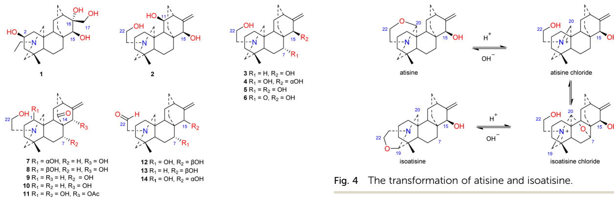
Fig. 2 The amine subtype of atisines.
