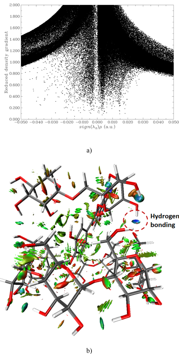
Fig. 9 Scatter graph of dependence of RDG on sign \lambda_2 ( \rho ) function (a); the RDG isosurface depicted at an isovalue of 0.8 of IIB complex (b).
