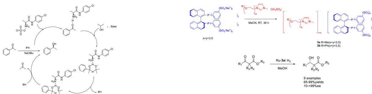
Scheme 3 Synthesis and application of phosphine functionalized chiral polyether ionic liquid in asymmetric catalytic hydrogenation reaction.
