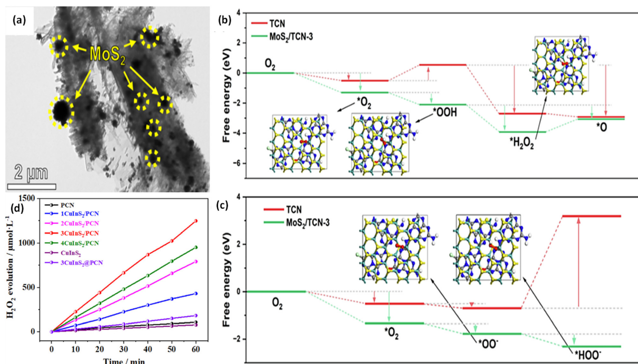
Fig. 27 (a) SEM images of \text{MoS}_2 -TCN-3. Free energy change graphs for the ^*\text{HO}_2^- 2e^- ORR pathway under (b) acidic and (c) alkaline conditions. The figures are adapted with permission from ref. 201. Copyright 2023, Elsevier. (d) Photocatalytic \text{H}_2\text{O}_2 generation by PCN, \text{CuInS}_2 , 3\text{CuInS}_2@ PCN, and x\text{CuInS}_2@ PCN samples. The figures are adapted with permission from ref. 202. Copyright 2023, Elsevier.
