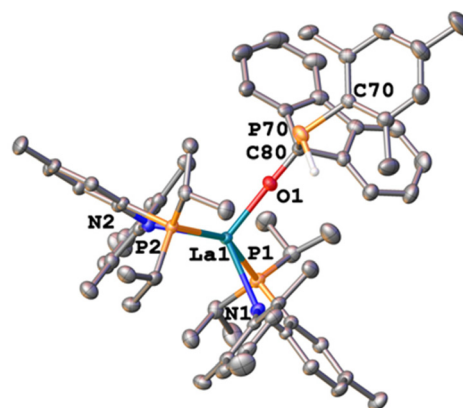
Fig. 2 Molecular structure of the hemiphosphinal complex 2a . Thermal ellipsoids are shown at a probability level of 50%. Hydrogen atoms (except for H70 on P70) and lattice solvent molecules have been omitted for clarity. Selected bond parameters of the hemiphosphinal moiety: 2a : La1–O1 2.1867(13) Å, O1–C80 1.401(2) Å, C80–P70 1.9163(19) Å, La1–O1–C80 177.79(12)°, O1–C80–P70 103.22(12)°.
