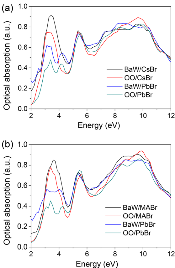
Fig. 6 Absorption coefficients of the relaxed perovskite/BaWO 4 interfaces: (a) CsPbBr 3 /BaWO 4 and (b) MAPbBr 3 /BaWO 4 .
