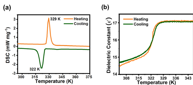
Fig. 2 (a) The DSC curve of 1 and (b) the dielectric constant curve of 1 at 1000 kHz.
