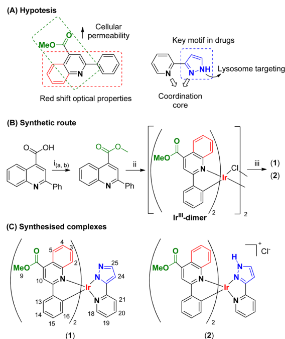
Fig. 2 (A) Hypothesis-based approach to probe design. (B) Synthetic pathway to prepare 1 and 2. (i) SOCl 2 , MeOH, (0 °C); (ii) reflux, 2 h; (iii) IrCl 3 ·nH 2 O, 2-ethoxyethanol, reflux, 24 h; (iii) 1) 3-(2-pyridyl)pyrazole, Cs 2 CO 3 , DCM, 318 K, 20 h; (iii) 2) DCM : MeOH (1 : 1), 298 K, 24 h. (C). Synthesised cyclometallated Ir III complexes.
