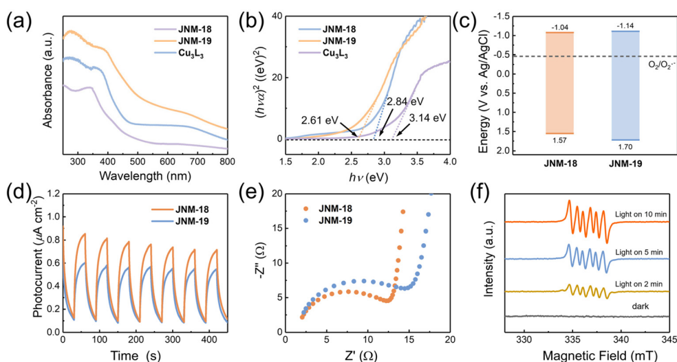
Fig. 4 (a) UV-Vis diffuse reflectance spectra of JNM-18 , JNM-19 and \text{Cu}_3\text{L}_3 . (b) Tauc plots of JNM-18 , JNM-19 and \text{Cu}_3\text{L}_3 based on the UV-Vis diffuse reflectance spectra obtained from the Kubelka–Munk function. (c) Schematic depiction of optical band gaps of JNM-18 and JNM-19 . (d) Photocurrent responses of JNM-18 and JNM-19 . (e) Electrochemical impedance spectra of JNM-18 and JNM-19 . (f) EPR spectra of JNM-18 with DMPO in MeCN in the dark or under light irradiation.
