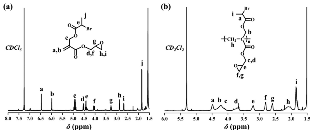
Fig. 1 ^1\text{H} NMR spectra of (a) the Br-acrylate-epoxide functional monomer and (b) the poly(Br-acrylate-epoxide) macro-agent.
