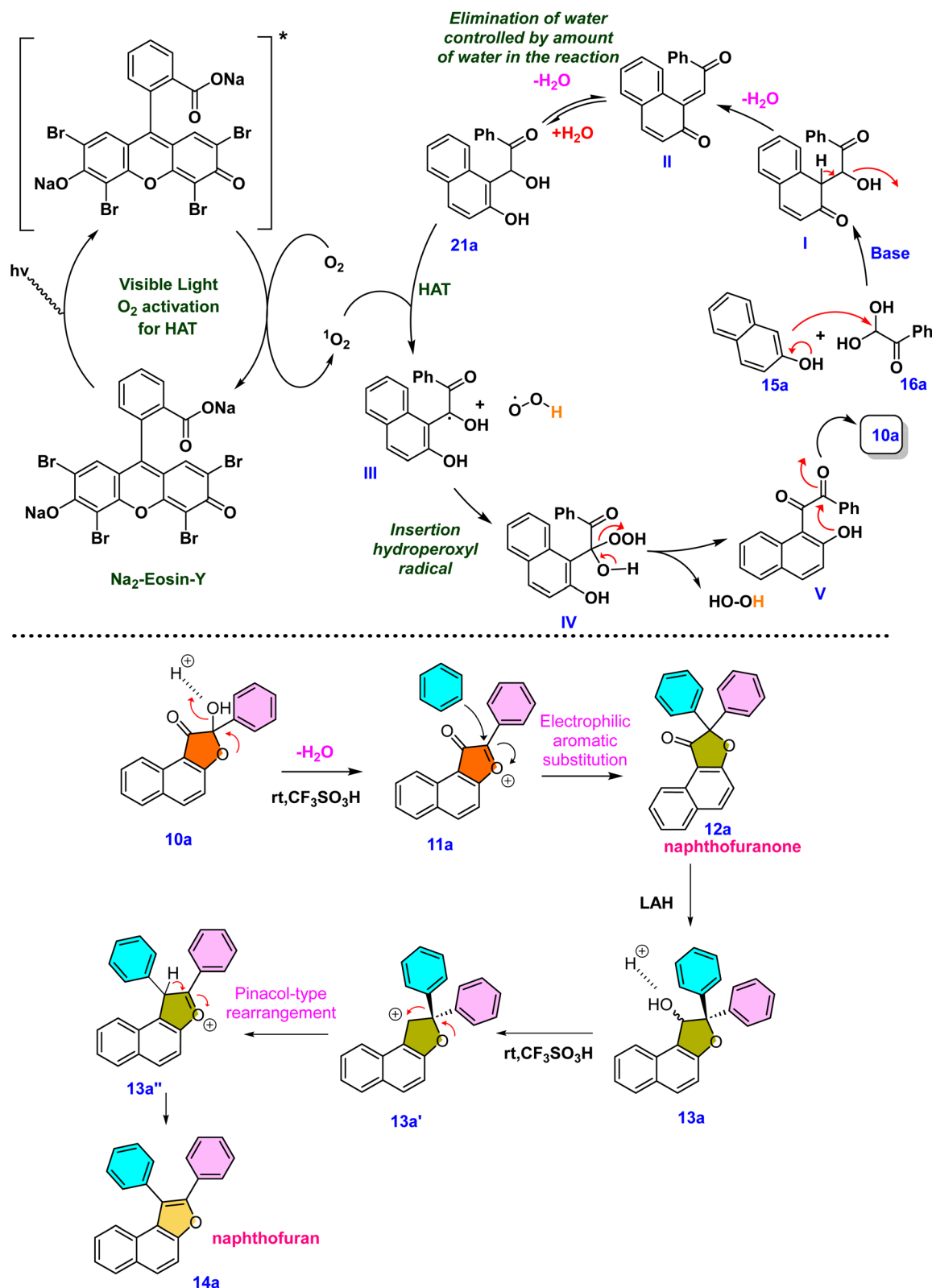
Scheme 7 Plausible mechanism.
