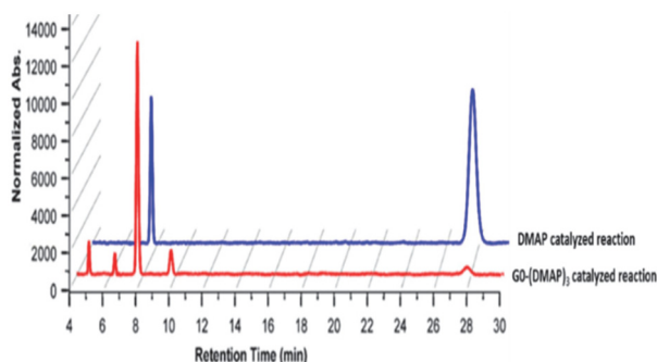
Fig. 1 HPLC chromatograms for the acetylation of glucopyranoside 40 . Chromatography conditions: Shimadzu Shim-pack (UC-X-Sil) 5\ \mu\text{m} column, \text{EtOAc} –hexane = 60 : 40, flow rate 1\ \text{mL min}^{-1} , PDA detector (254 nm), retention times: 7.6 min (major isomer 41 ), 27.7 min (starting material 40 ) and the remaining peaks correspond to the minor isomers.
