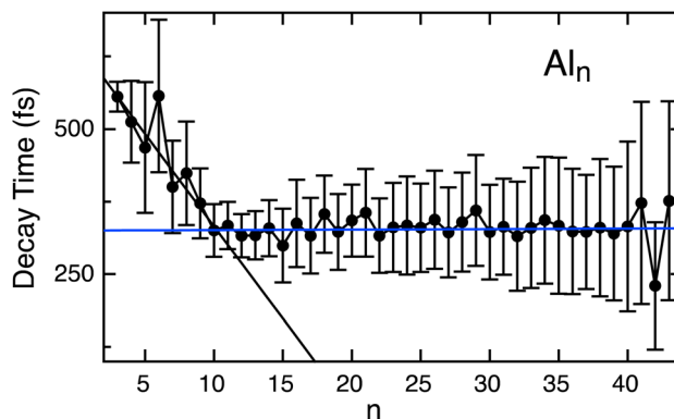
Fig. 3 Excited state lifetimes of \text{Al}_n ( n = 3\text{--}43 ) decrease with size for n < 10 , and then plateau for larger clusters reaching an average value of 327 fs. The black trend line corresponds to the fit of \text{Al}_3\text{--Al}_{10} , whereas the blue line is the fit of \text{Al}_{11}\text{--Al}_{43} .
