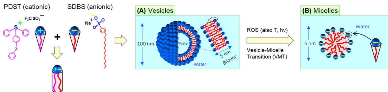
Fig. 1 Concept behind this study: vesicle–micelle transitions (VMTs) induced by ROS, heat, and light. The cationic amphiphile PDST and the anionic surfactant SDBS are combined to produce the vesicles. Each molecule has a cone-like geometry, but their mixtures are cylinder-shaped (due to electrostatic binding of their heads). Self-assembly leads to “catanionic” vesicles with sizes \sim 100 nm (A). Each vesicle has a 5 nm-thick bilayer membrane enclosing an aqueous core. When contacted with ROS, the vesicles undergo a VMT (B). The resulting micelles are \sim 5 nm in size and have a hydrophobic core. A VMT can also be induced by heat as well as irradiation with UV light.
