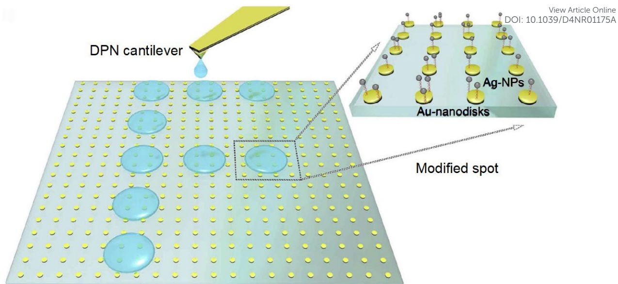
Figure 6: Schematic illustration of the fabrication process of plasmonic nanostructures.
