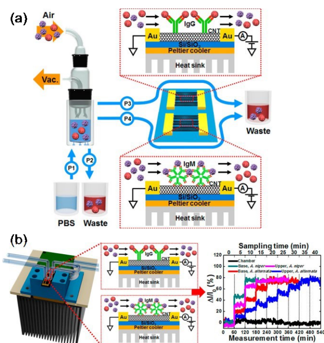
Figure 14: (a) Schematic diagram of the bioaerosol auto-monitoring instrument (BAMI) integrated with a bioaerosol sampler and two-channel carbon nanotube field-effect transistors (CNT-FETs) for real-time monitoring of airborne fungal particles. (b) Illustration of CNT-FET functionalization with specific antibodies for capturing airborne Aspergillus niger and A. alternata particles, resulting in changes in electrical conductivity for immediate analysis. Reprinted with permission from ref. [74] (copyright © 2016 Published by American Chemical Society).
