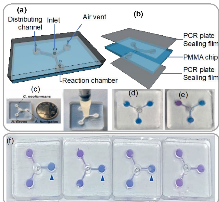
Figure 18: (a) Description of the apparatus (b) assembly of the chip (c) three sets of primers were preloaded with 0.5% low melt agarose in the reaction chamber (d) The chip's adapter (e) Verification of the possibility and cross-contamination of LAMP assays implemented on the microfluidic chips (f) Outcomes of the colorimetric LAMP assays conducted on the chips at 4 \times 10^6 , 4 \times 10^5 , 4 \times 10^4 and 4 \times 10^3 spores per sample. Reprinted with permission from ref. [50] (copyright © 2022 Published by Elsevier B.V.).
