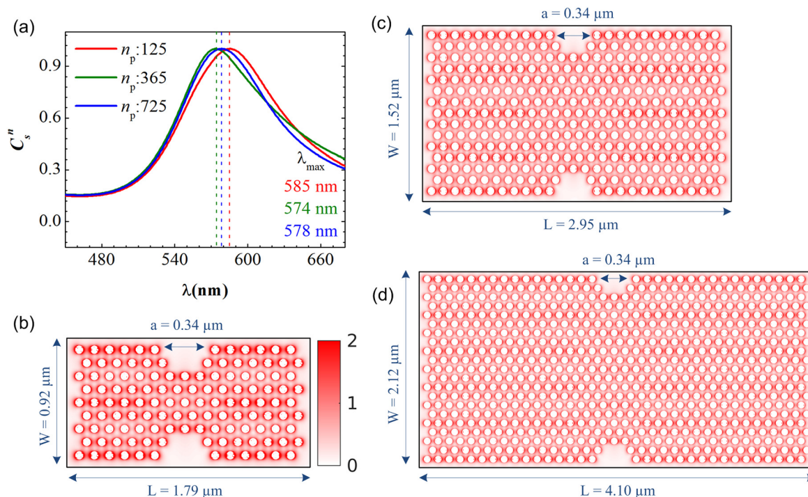
Fig. 2 (a) Normalized scattering cross section, C_s^n , as a function of wavelength for three PGP arrays composed of 125 (red curve), 365 (green curve) and 725 (blue curve) PGP particles. Electric field amplitude on the xy -plane (where z = 0 ) for the arrays with (b) 125, (c) 365 and (d) 725 PGP particles. The structure is illuminated with an X-polarized plane wave propagating in the z direction. The electric field maps are calculated at the resonance wavelengths, \lambda_{\max} .
