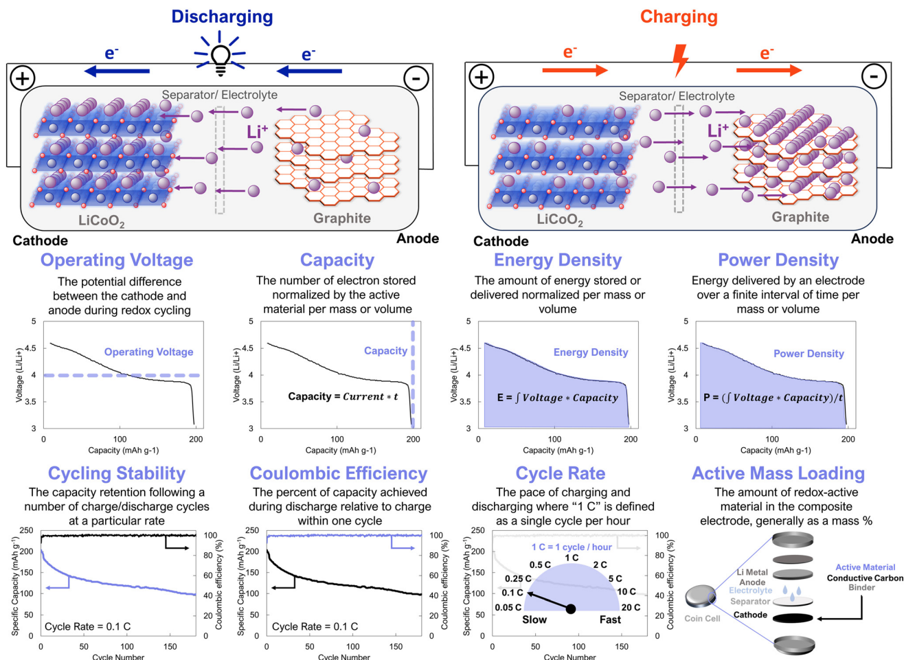
Fig. 1 Schematic of battery charging/discharging processes and common performance metrics to evaluate new electrode active materials. Data is for LiCoO 2 , which was adapted with permissions from ref. 5. Copyright © 2022 Wiley.
