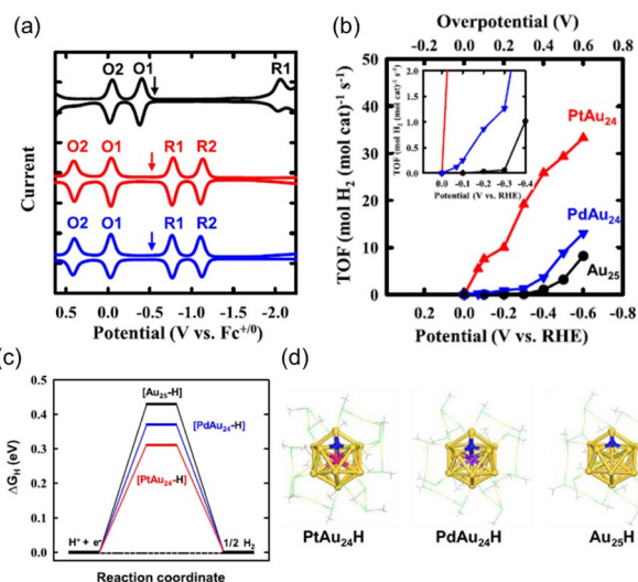
Fig. 3 (a) Square-wave voltammetry (SWV) of MAu 24 (SC6) 18 with M = Au (black), Pt (red), and Pd (blue) in dichloromethane (1.0 mM). The arrows denote the open circuit potential of the NCs. (b) Turnover frequency (TOF) against the potential obtained from the constant potential electrolysis of the MAu 24 (SC6) 18 /C/gas diffusion layer electrode in 1.0 M Britton–Robinson buffer solution containing KCl (2.0 M). Inset: enlarged view of the low-overpotential region. (c) Hydrogen adsorption Gibbs free energy ( \Delta G_{\text{H}} ) diagrams for MAu 24 (SCH 3 ) 18 obtained by theoretical calculations and (d) DFT-optimised structures of H-MAu 24 (SCH 3 ) 18 . Color code: pink, Pt; purple, Pd; yellow, Au; blue, adsorbed H. Protection motifs are in the line view; green, S; gray, C; white, H. Reproduced from ref. 47 with permission from the American Chemical Society, Copyright 2018.
